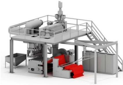
Meltblown Fabric Making line Routine vertical Costly
